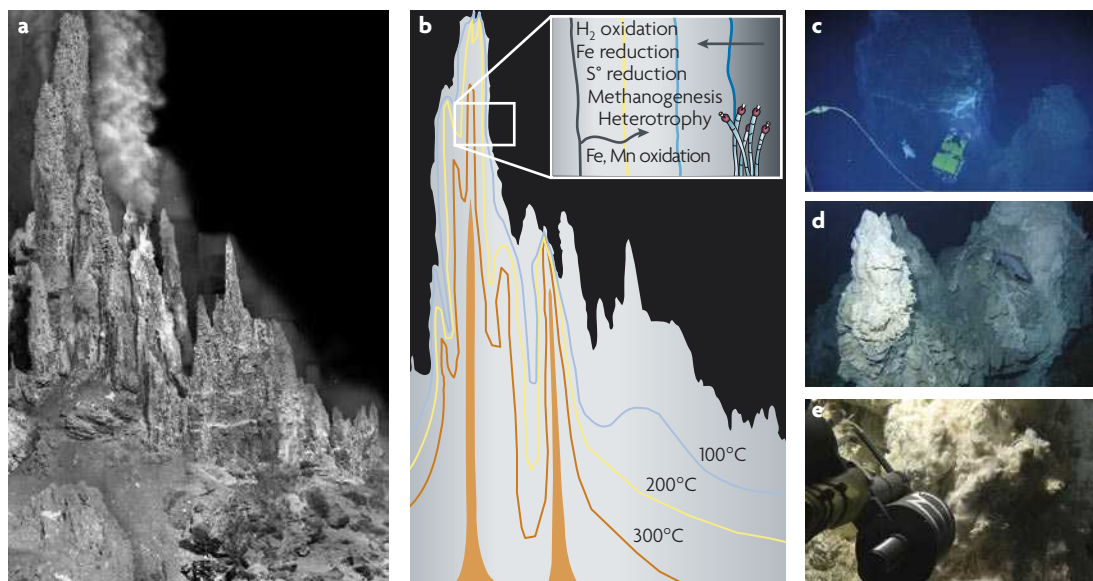
Figure 2 | Hydrothermal vents. There are two main types of hydrothermal vent: the black smoker type (a,b) and the Lost City type (c–e). a | A black smoker in the Faulty Towers complex in the Mothra hydrothermal field on the Endeavour Segment of the Juan de Fuca Ridge. The tallest chimney rises 22 metres above the sea-floor. The ‘furry’ appearance of the chimneys reflects the fact that the chimney walls are encrusted in dense communities of tube worms, scale worms, palm worms, sulphide worms and limpets. The two-pronged chimney in the middle with an active plume is a 300°C chimney called Finn, from which a 121°C organism was cultured that uses Fe(III) as an electron acceptor in the presence of N 2 and CO 2 (REF. 15). b | The outer surface of black smoker chimneys is bathed in a mixture of 2°C, oxygenated sea-water and warm vent fluid that escapes from within the structure. The inner walls that form the boundary of the central up-flow conduits commonly exceed 300°C, and temperatures are fixed by a steady supply of rapidly rising, strongly reducing vent fluid. Intermediate conditions exist as gradients between these extremes. Changes in microbial abundance, diversity and community structure have been associated with inferred environmental gradients in the chimney walls 99,100 . c | Microbial sampling at the Lost City hydrothermal field. The robotic vehicle Hercules is shown hovering near the summit of the 60-metres-tall Poseidon complex. White areas are active or recently active sites of venting. d | The top left part of the Nature Tower. Wreck-fish, which are ~1 metre in length and are commonly found at a water depth of 750 metres, routinely investigated the vehicles. The Poseidon complex has four pinnacles, two of which are shown here. Actively venting edifices are composed of aragonite (CaCO 3 ) and brucite (Mg(OH) 2 ). The grey–brown material also contains carbonate, but is richer in calcite that has recrystallized from aragonite. e | A close up of a 75°C, diffusely venting carbonate chimney showing a titanium water sampler. Dense colonies of filamentous bacteria thrive in the high pH, CH 4 - and H 2 -rich fluids. The insides of the chimneys are dominated by a single phylotype of archaea from the Methanosarcinales order that grow at 80°C. A phylotype of anaerobic methanotrophic archaea are restricted to lower-temperature chimneys. Bacterial 16S ribosomal RNA gene sequences correspond to a diverse community that includes species of Methylobacter (or Methylomonas ), species of Thiomicrospira , members of the Firmicutes phylum and Desulfotomaculum alkaliphilus 28 . Parts a,b courtesy of D. Kelley and J. Deloney, University of Washington, USA. Images c–e courtesy of D. Kelley, Institute for Exploration, University of Rhode Island, USA, and the National Ocean and Atmospheric Administration Office of Ocean Exploration.
